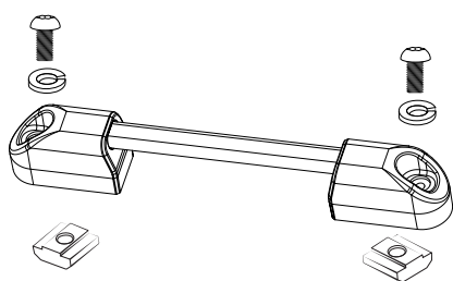
5. Handle + Bolts + Spring washer | x1 set
