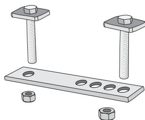
3. Vehicle connection brackets Stainless steel lock plates | x 4 sets
